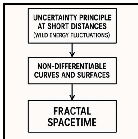
Fig. 1. From the uncertainty principle to fractal spacetime
