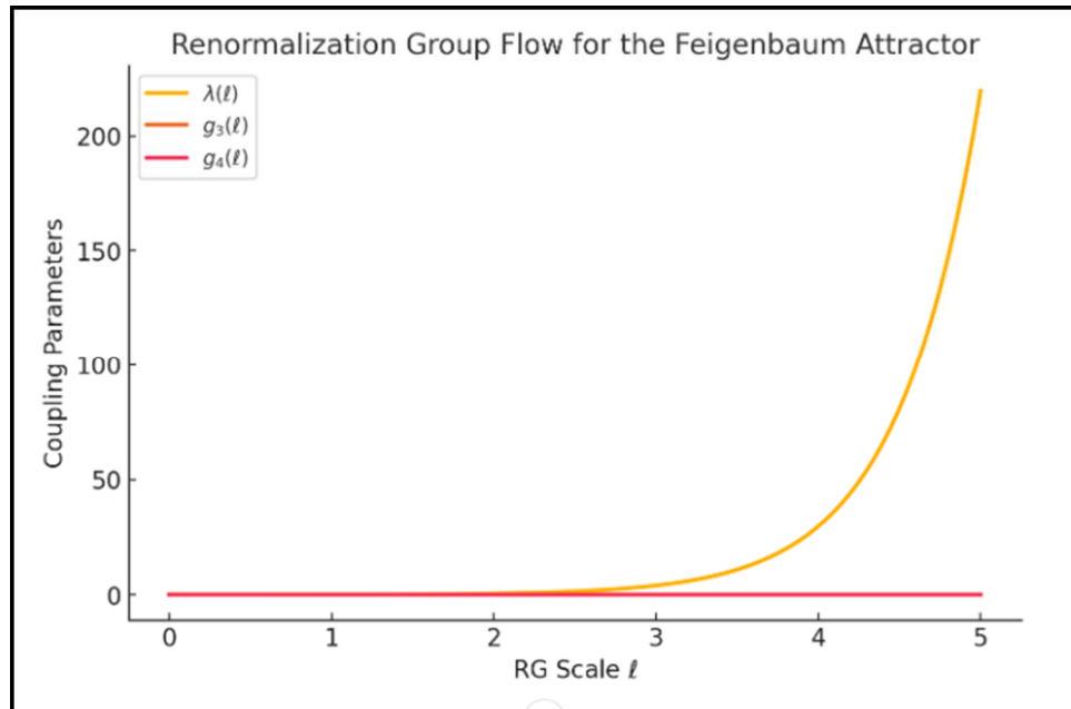
Fig. 3. RG plot of coupling parameters for the quadratic map
