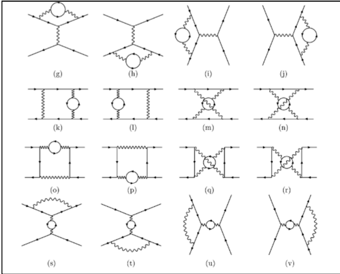
Fig. 1. Feynman diagrams containing vertices, lines and loops.
