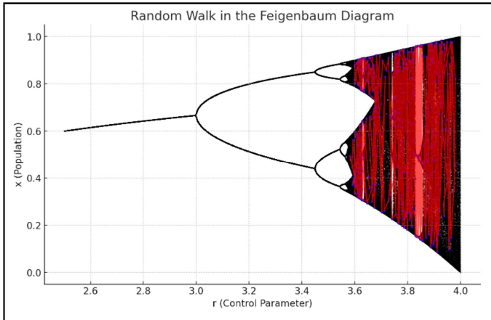
Fig. 2. Visualization of random walks on the bifurcation diagram
